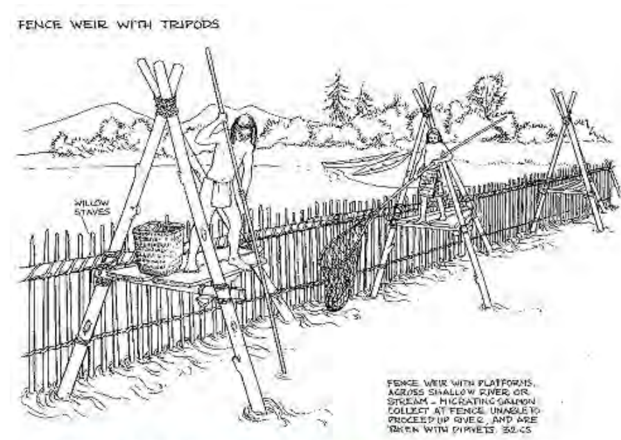
Drawing of a First Nations fence weir with tripods. Image © Hilary Stewart. Indian Fishing: Early Methods on the Northwest Coast , p. 104.
